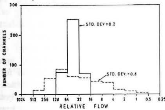
Figure 10 - Channel network (CN) model and advection-dispersion (AD) model comparison
