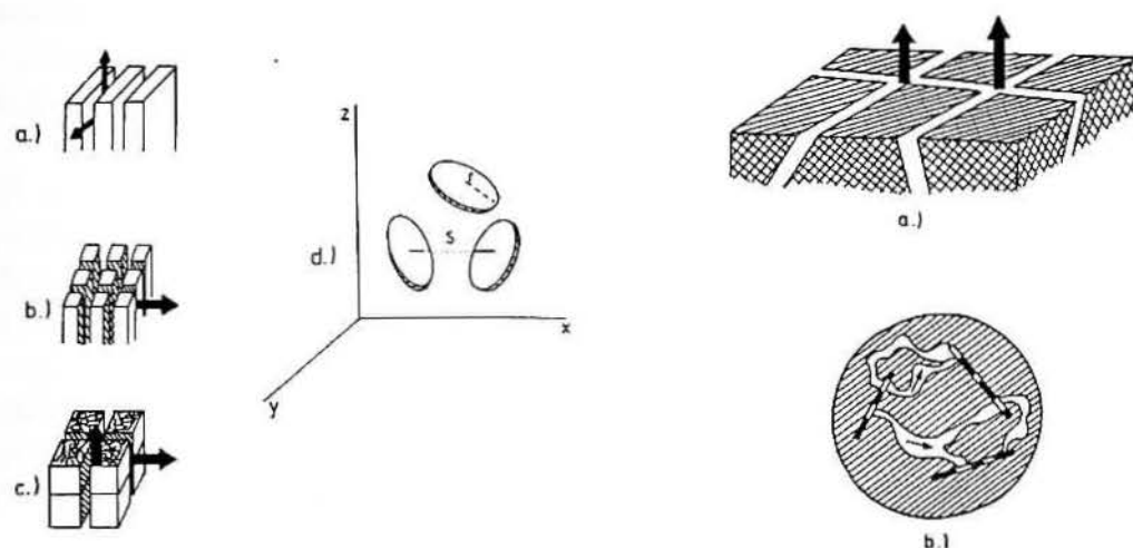
Figure 8 - Some examples of discrete flow models Orthogonal models (left): a) parallel, b) matchstick, c) cubic; Disc models (centre): d) Beacher disc model; Channel network models (right): a) channels at fracture sections, b) channels within fractures
