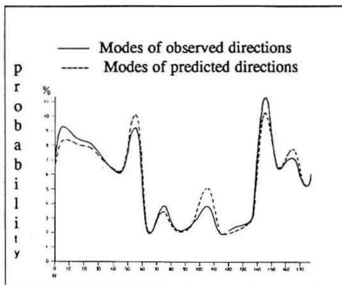
Figure 4 - Comparison between the observed and calculated directional frequencies of the active karst drainage channels in Libar, Spain (after Eraso,1986)
