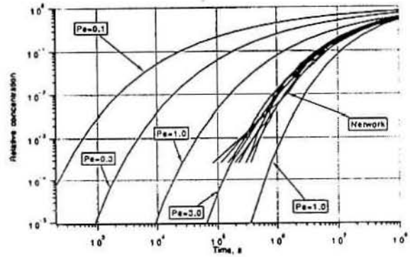
Figure 10 - Channel network (CN) model and advection-dispersion (AD) model comparison
